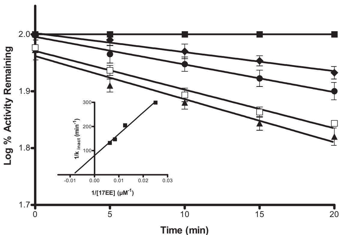
Fig. 5. Inactivation of P450 2B6.4 by 17EE in the presence of cytochrome b_5 . The time- and concentration-dependent inactivation of P450 2B6.4 by 17EE was measured by determining the 7-EFC O -deethylation activity. After initiation of the reaction by the addition of NADPH, aliquots were removed from the primary reaction mixture at 0, 5, 10, 15, and 20 min. The concentrations of efavirenz were 0 \mu M (■), 40 \mu M (◆), 80 \mu M (●), 120 \mu M (□), and 160 \mu M (▲). The data show the means and standard deviations from four separate experiments done in duplicate. In some cases the standard deviations were less than the size of the symbols. The inset shows the double reciprocal plot of the rates of inactivation as a function of the 17EE concentrations.
