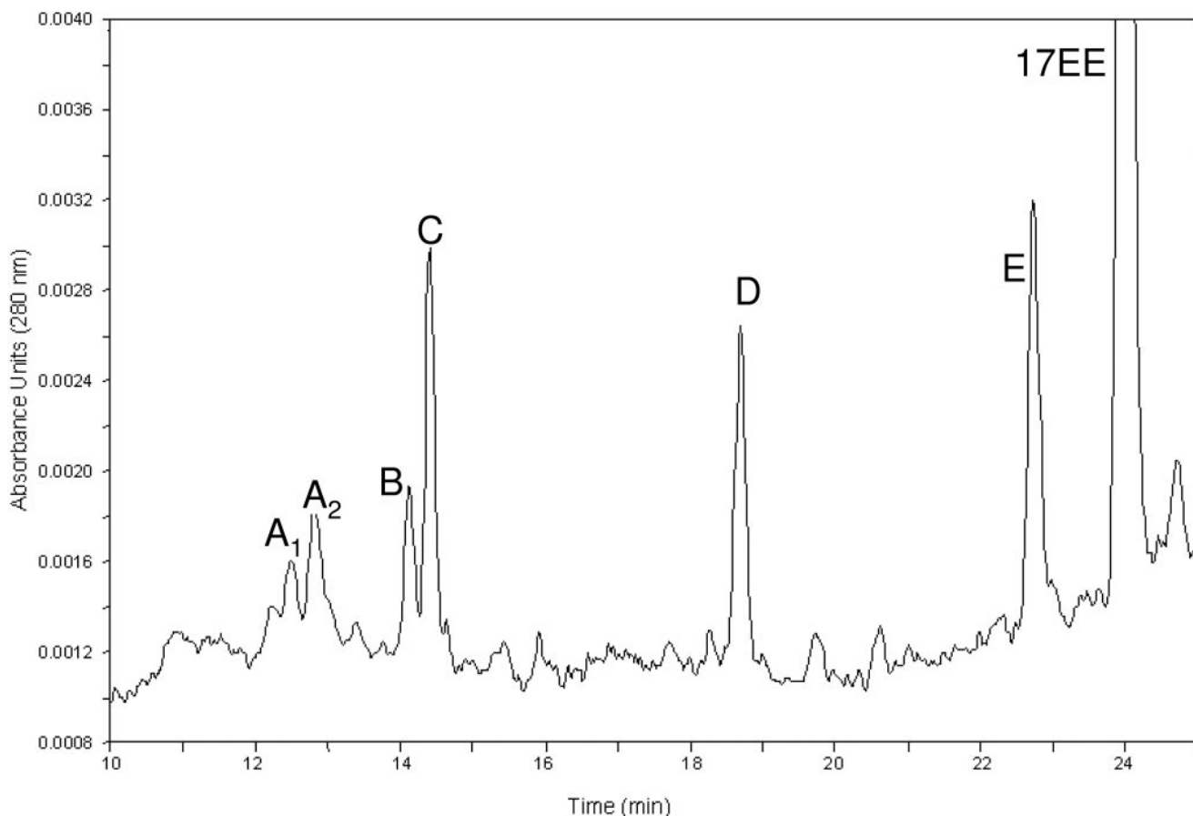
Fig. 6. Metabolism of 17EE by P450 2B6.4 in the presence of cytochrome b_5 . Metabolites A 1 , A 2 , and C are monohydroxylated metabolites, although the exact identities have not yet been determined. Metabolite D corresponds to 2-hydroxy-17EE; metabolite E corresponds to estrone. The parent compound, 17EE, is labeled. We previously showed that in the absence of cytochrome b_5 , P450 2B6.4 does not readily metabolize 17EE (Bumpus et al., 2005).
