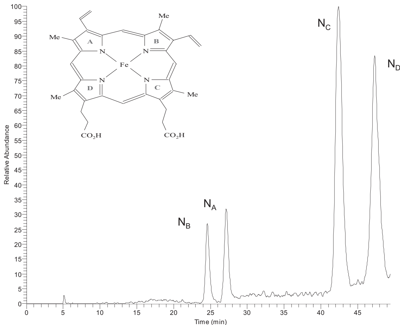
Fig. 2. Formation of P450 2B6 N -phenylprotoporphyrin IX regioisomers. P450 2B6 was incubated with phenyldiazene and the phenyl-iron complex formation was observed spectrally as described under Materials and Methods . Oxidation caused migration of the phenyl to the porphyrin nitrogens. The individual peaks represent migration of the phenyl to pyrrole rings A ( N_A ), B ( N_B ), C ( N_C ), or D ( N_D ). Sample treatment and HPLC separation of the regioisomers were performed as described under Materials and Methods . The inset shows the heme structure with labeled pyrrole rings A, B, C, and D. The chromatograms are representative of three separate experiments.
