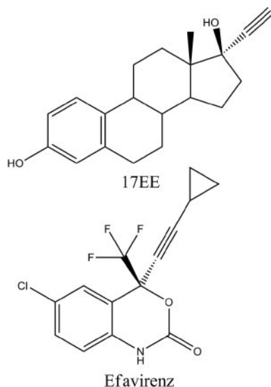
Fig. 1. Chemical structures of efavirenz and 17EE.
