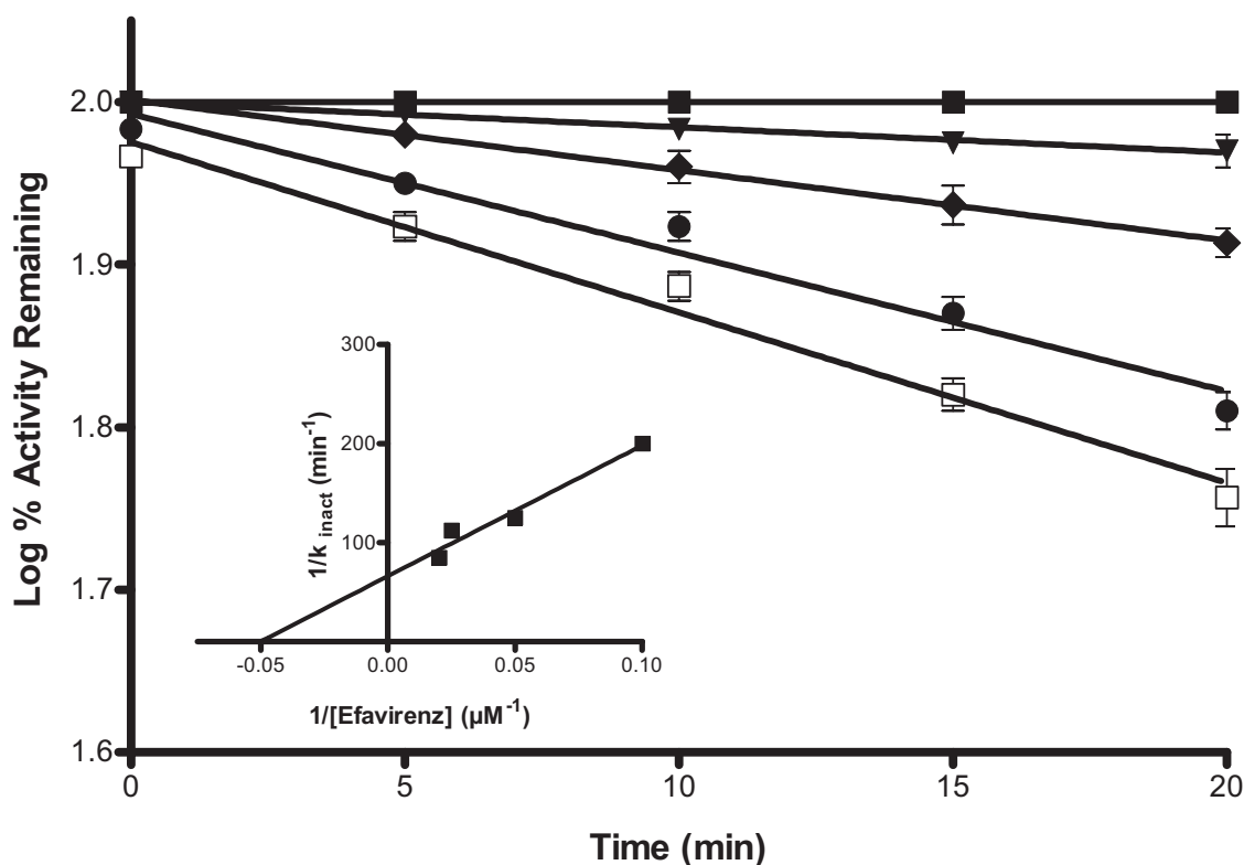
Fig. 4. Inactivation of P450 2B6.4 by efavirenz in the presence of cytochrome b 5 . The time- and concentration-dependent inactivation of P450 2B6.4 by efavirenz in the presence of cytochrome b 5 was measured by determining the 7-EFC O -deethylation activity. After initiation of reaction by the addition of NADPH, aliquots were removed from the primary reaction mixture at 0, 5, 10, 15, and 20 min. The concentrations of efavirenz were 0 μM (■), 10 μM (▼), 20 μM (◆), 40 μM (●), and 50 μM (□). The data show the means and standard deviations from four separate experiments done in duplicate. In some cases, the standard deviations were less than the size of the symbols. The inset shows the double reciprocal plot of the rates of inactivation as a function of the efavirenz concentrations.
