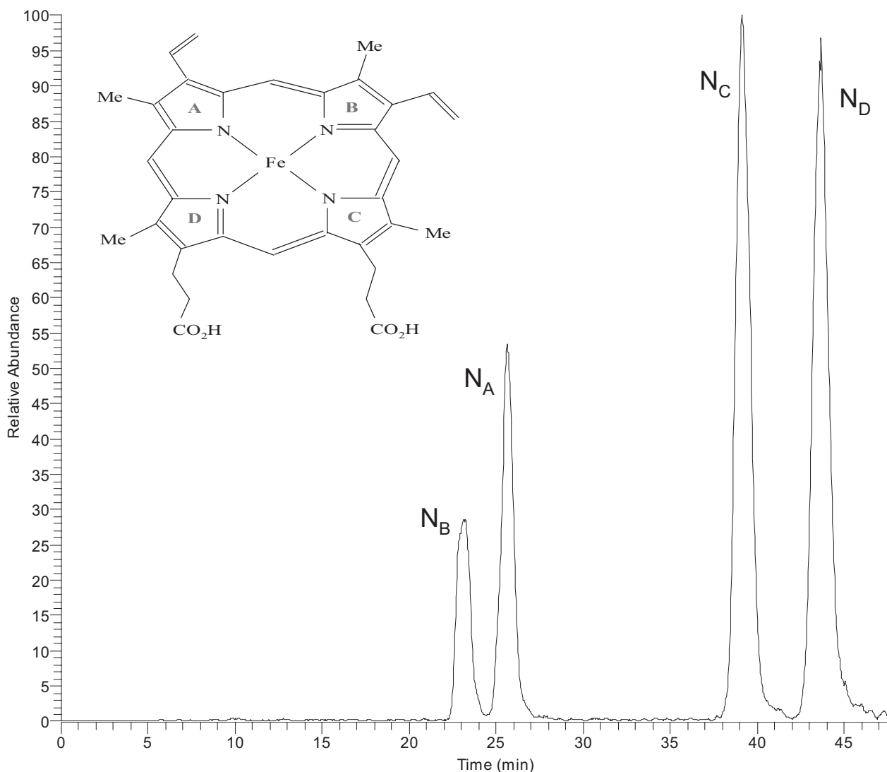
Fig. 3. Formation of P450 2B6.4 N -phenylprotoporphyrin IX regioisomers. P450 2B6.4 was incubated with phenyldiazene and the phenyl-iron complex formation was observed spectrally as described under Materials and Methods . Oxidation caused migration of the phenyl to the porphyrin nitrogens. The individual peaks represent migration of the phenyl to pyrrole rings A ( N_A ), B ( N_B ), C ( N_C ), or D ( N_D ). Sample treatment and HPLC separation of the regioisomers were performed as described under Materials and Methods . The inset shows the heme structure with labeled pyrrole rings A, B, C and D. The chromatograms are representative of three separate experiments.
